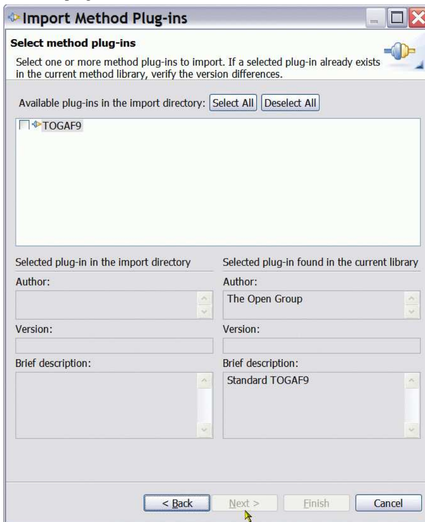
Figure 16. Method plug-ins
