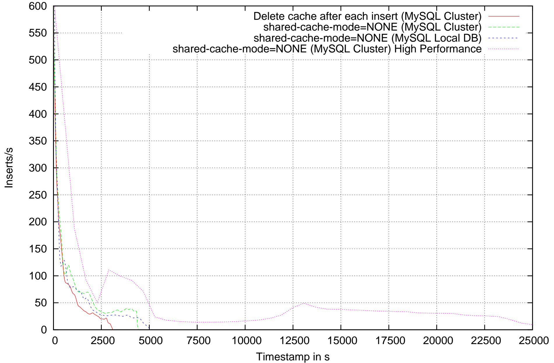
JPA (Eclipselink) Insert Test
